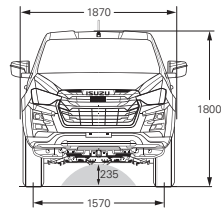
SX Space Cab Chassis 4x2 & 4x4
