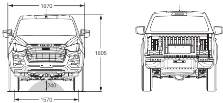
LS-U Crew Cab Chassis 4x4
