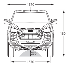
SX Crew Cab Chassis 4x2 & 4x4
