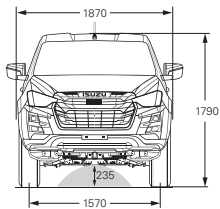
SX Single Cab Chassis 4x2 & 4x4
